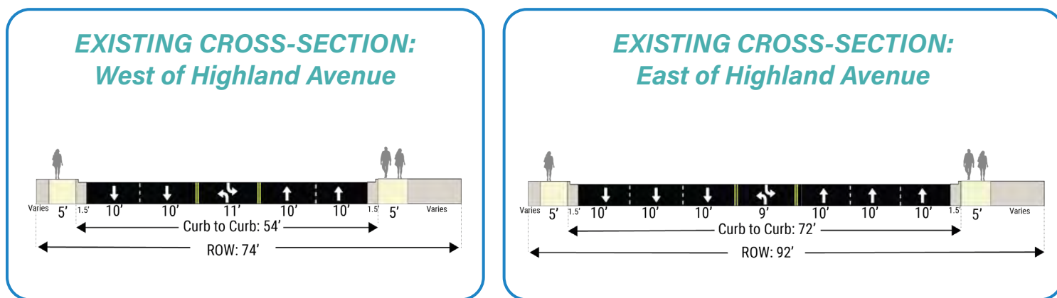
Figure 5.5: Existing Cross-Sections. NOTE: These cross-sections are not to scale.
