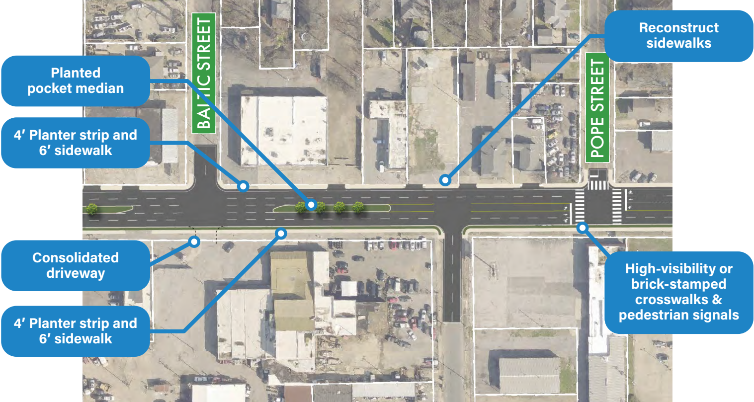
Figure 5.14: Conceptual design of the planted median near Pope Street.
