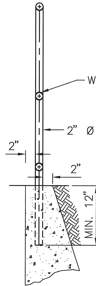
POST SET IN CONC. RETAINING WALL
