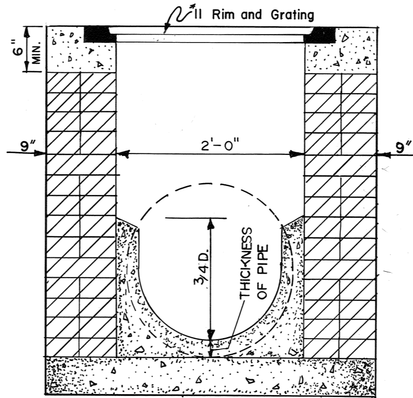
CROSS SECTION
