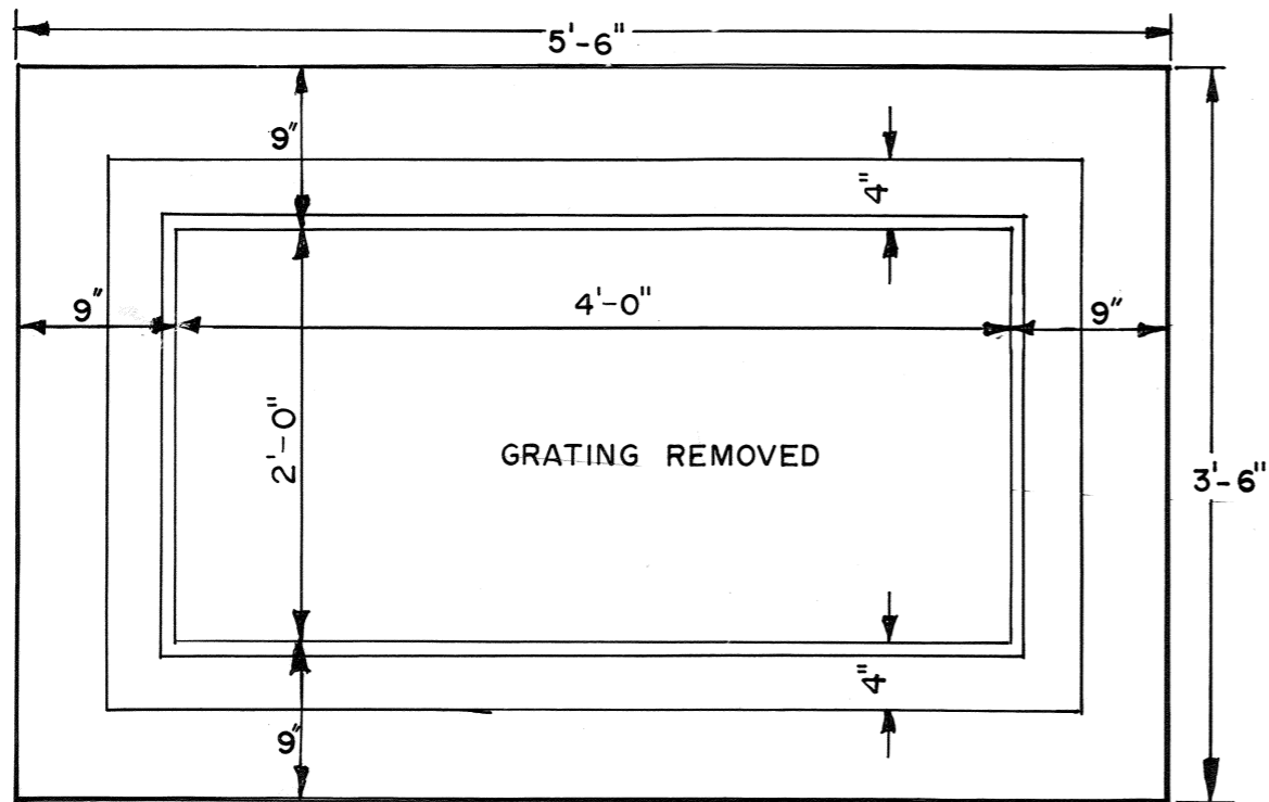
PLAN
