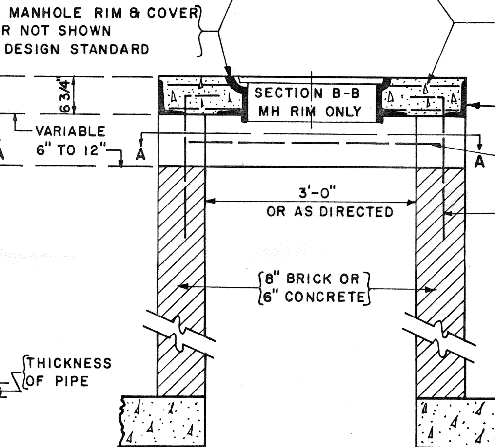
SECTION OVER CONCRETE BOX CULVERT
