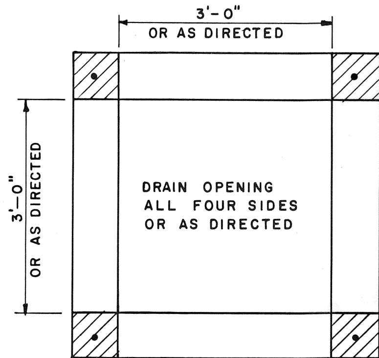
PLAN SECTION A-A
