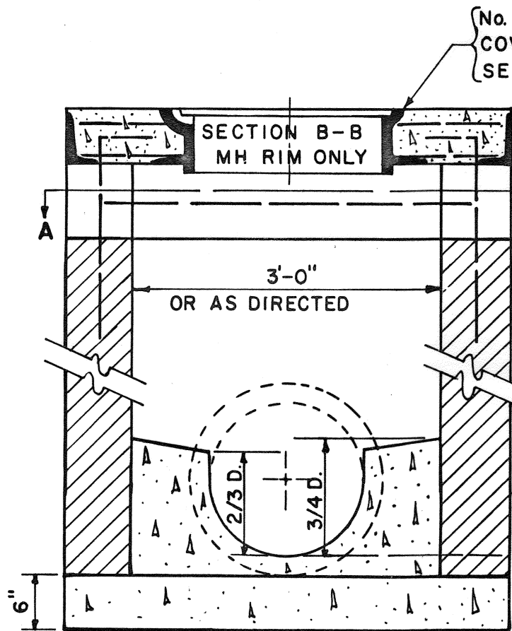
SECTION OVER PIPE
