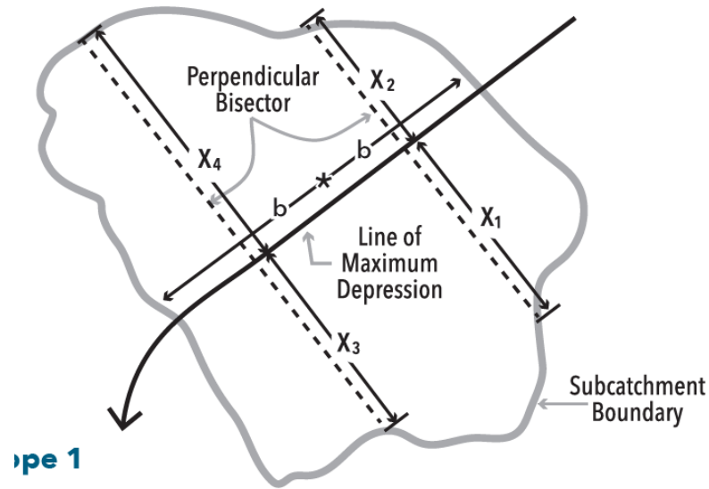
Figure 11 Determination of Basin Slope
